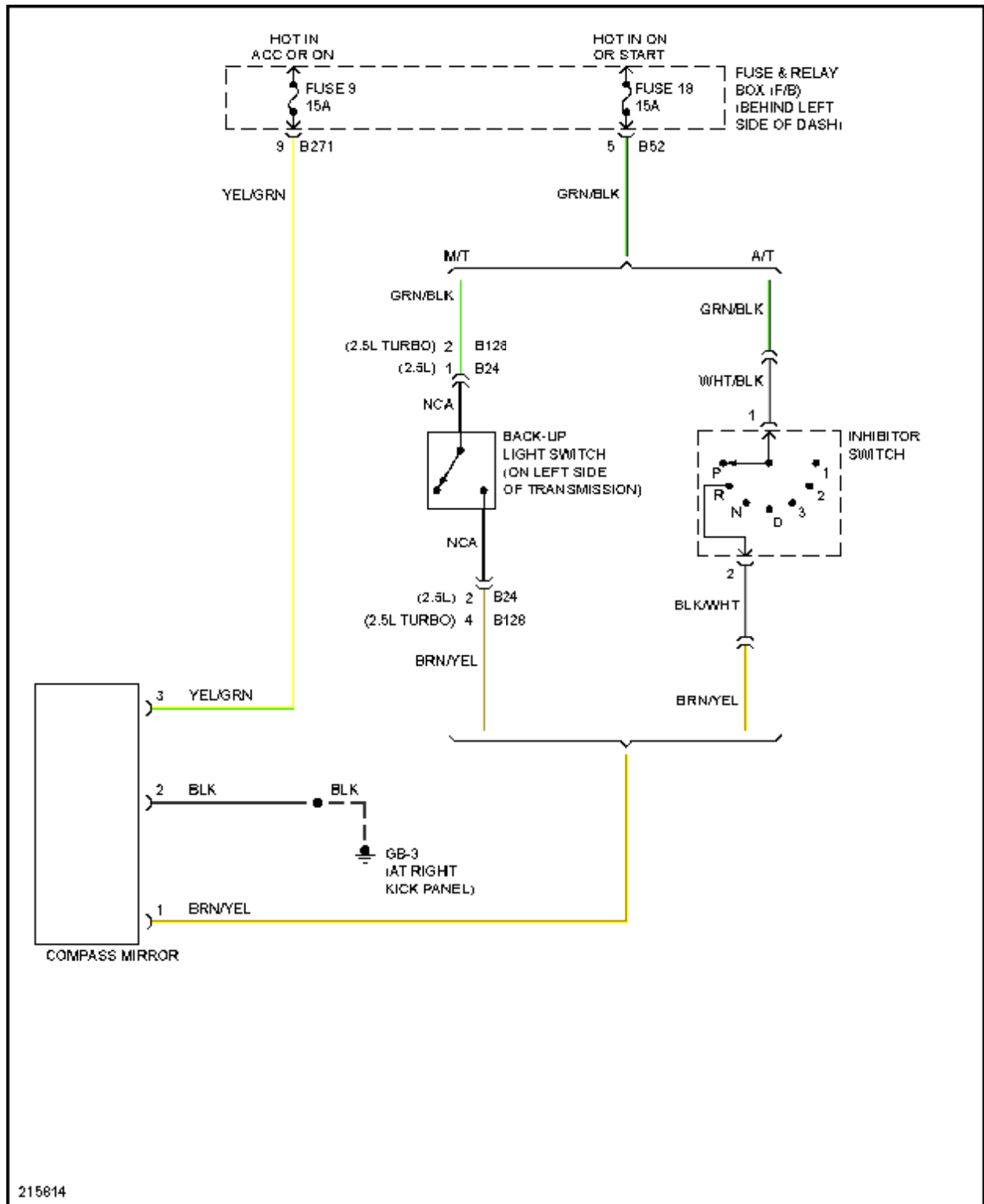
Fig. 40: Automatic Day/Night Mirror Circuit
